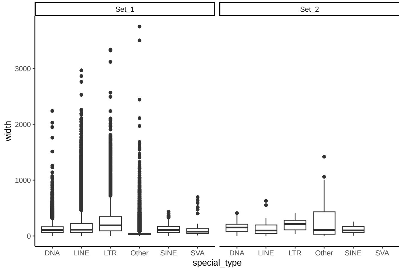
Minimum overlapping TE & ROI width length per class in H3K27me3
